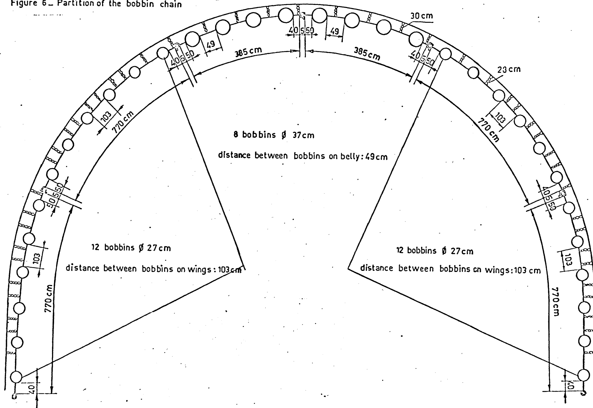
Figure 6 - Partition of the bobbin chain
