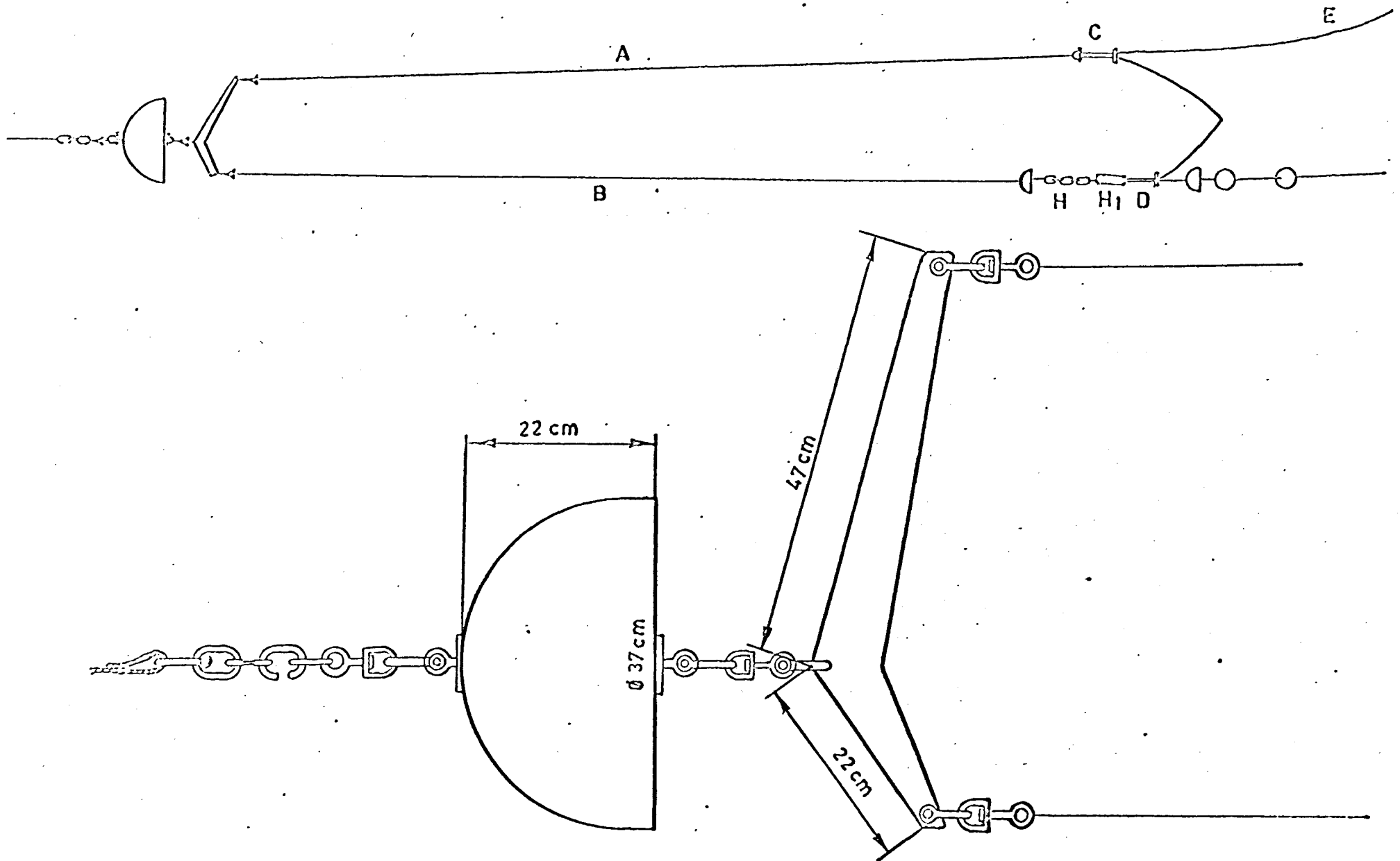
Figure 4 - Detail of the danleno and legs
