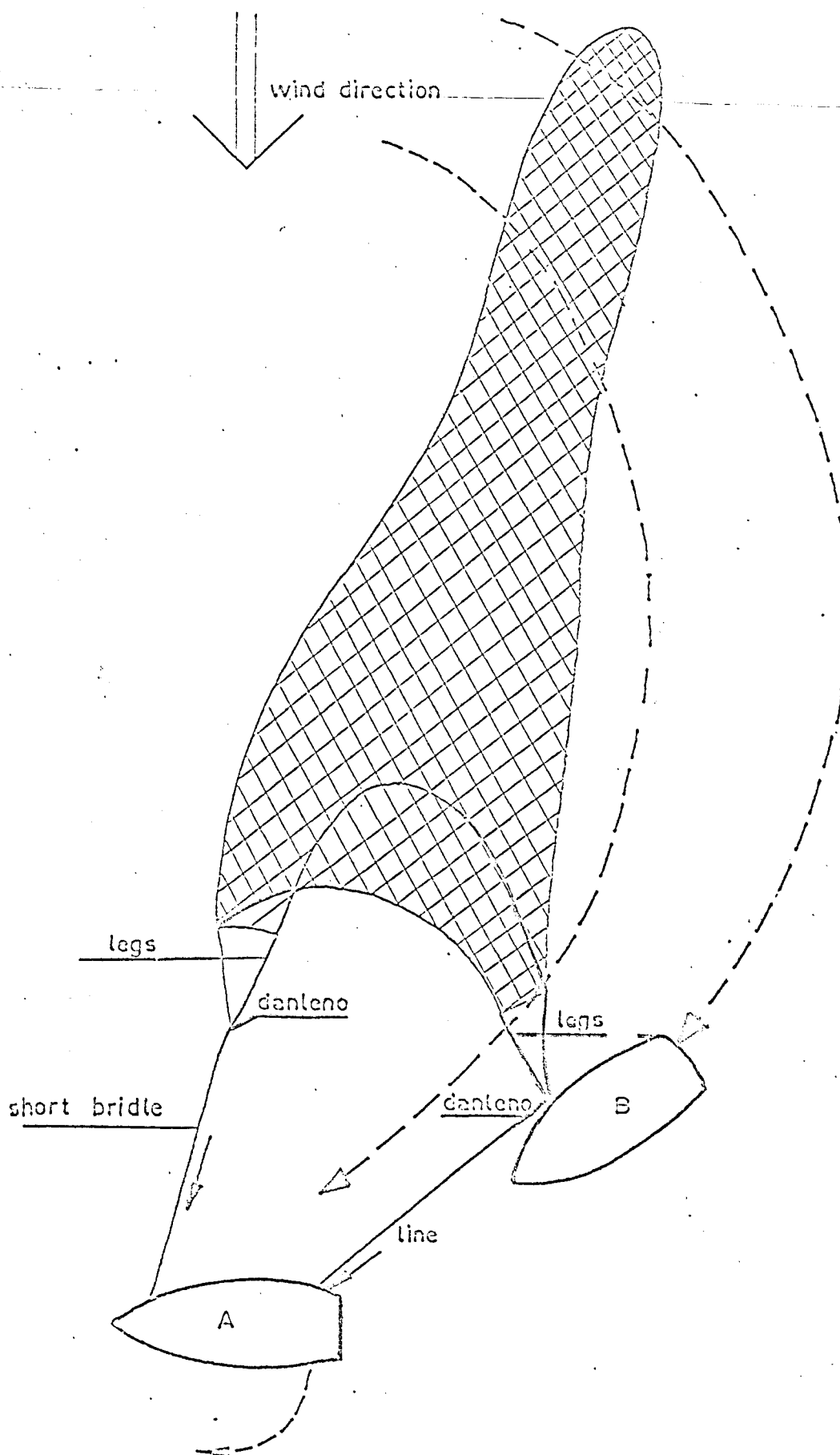
Figure 15 - Hauling: phase 4
