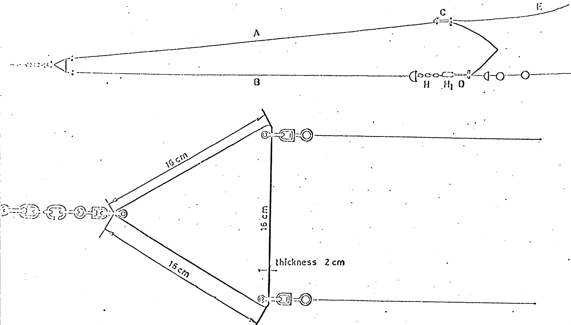
Figure 5 _ Detail of the triangle and legs
