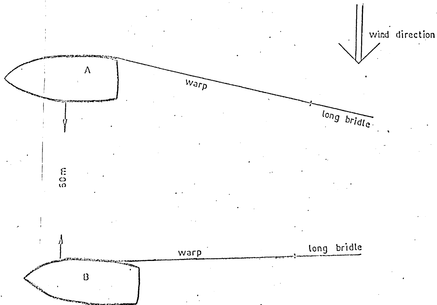
Figure 12 - Hauling: phase 3
